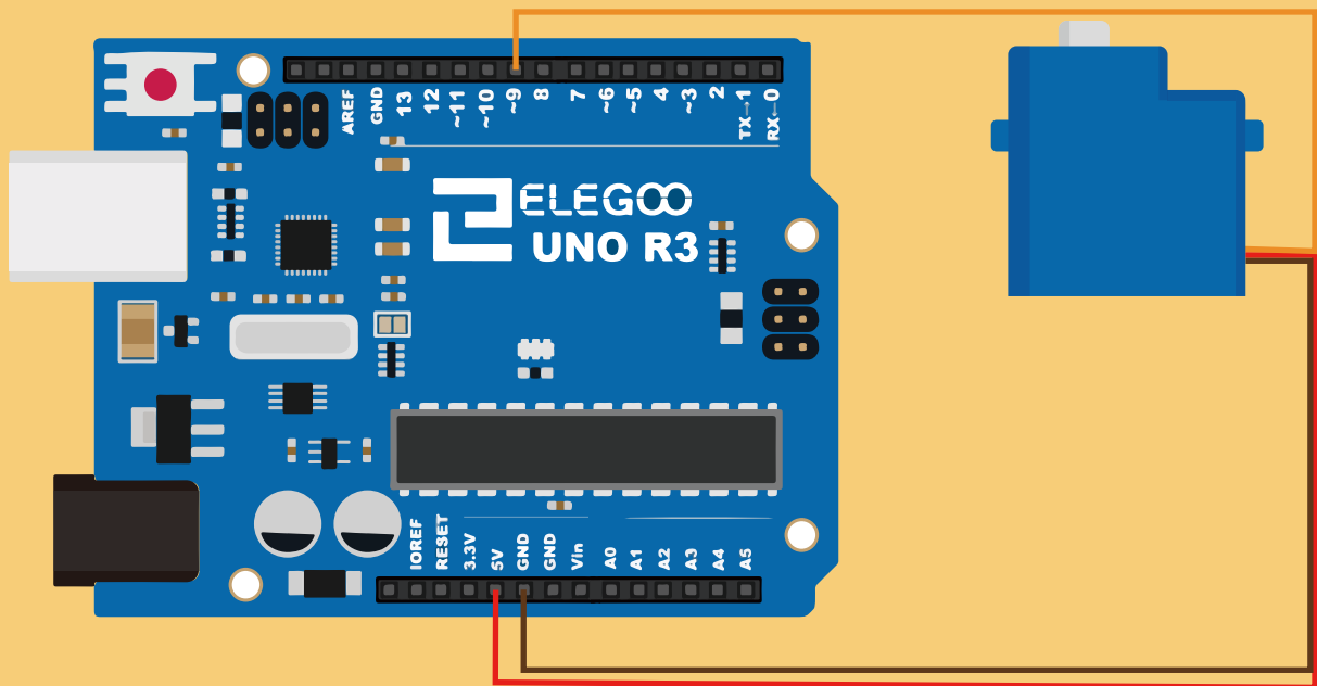
Wiring diagram
